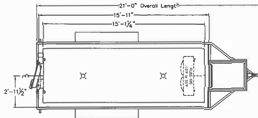
PLAN VIEW
