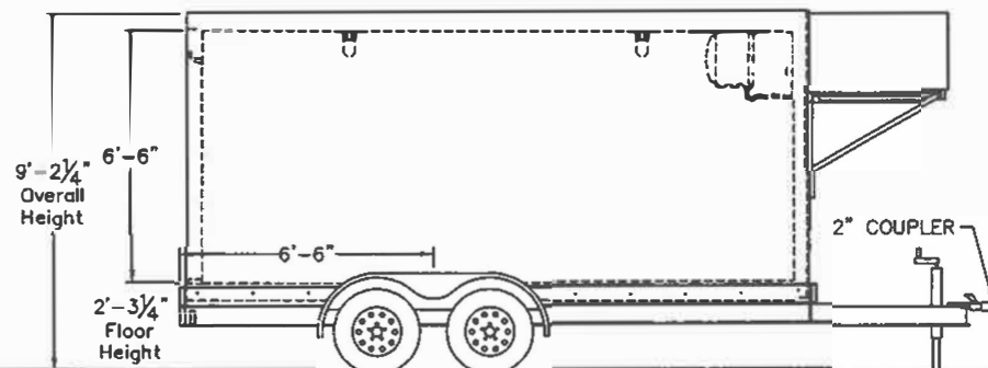
ELEVATION VIEW
