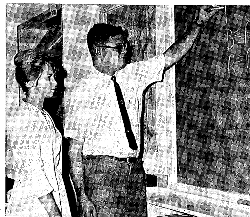
If P=R and B=P , then B=R .
